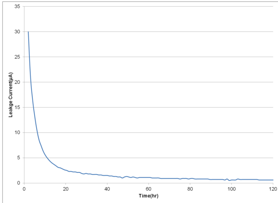
Fig 10: Leakage Current
