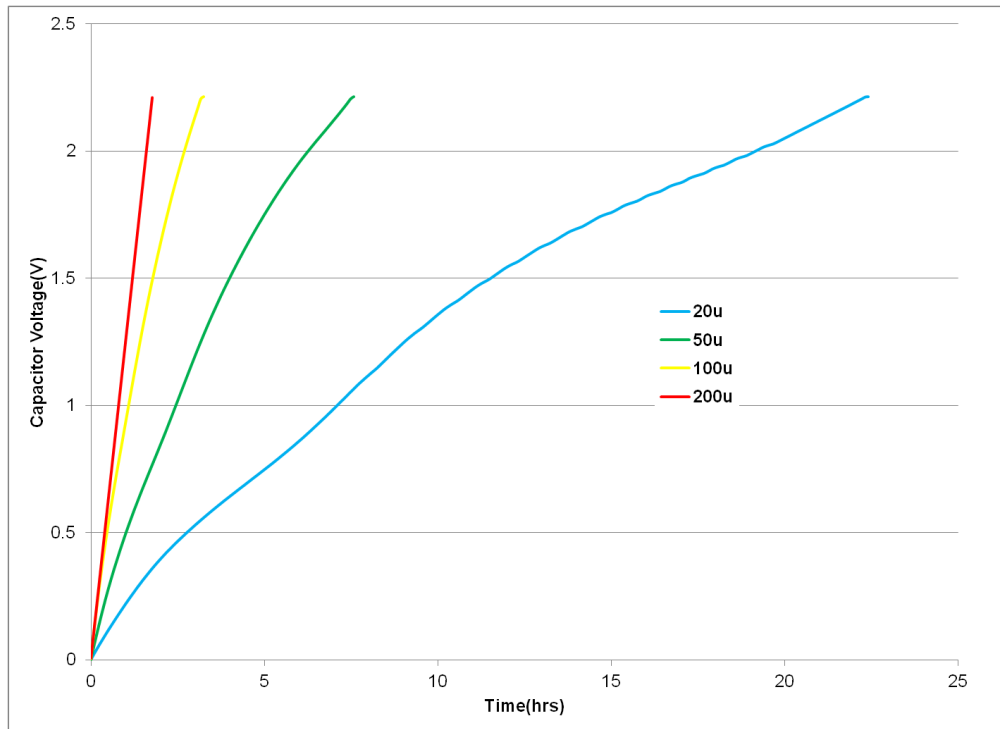
Fig 11: Charging an HA102 with low current
