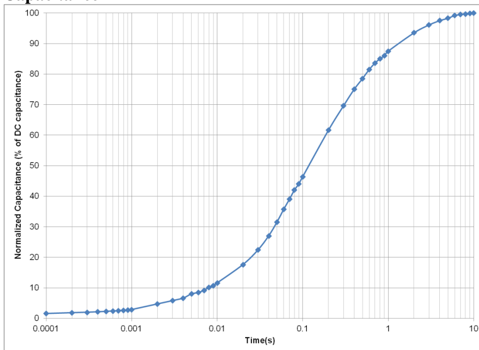
Figure 4: Effective Capacitance
