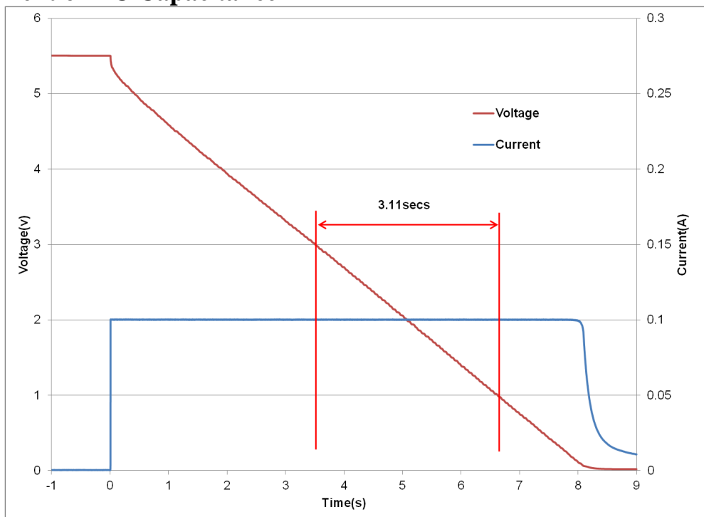
Fig 2: Measurement of DC Capacitance for an HA202
