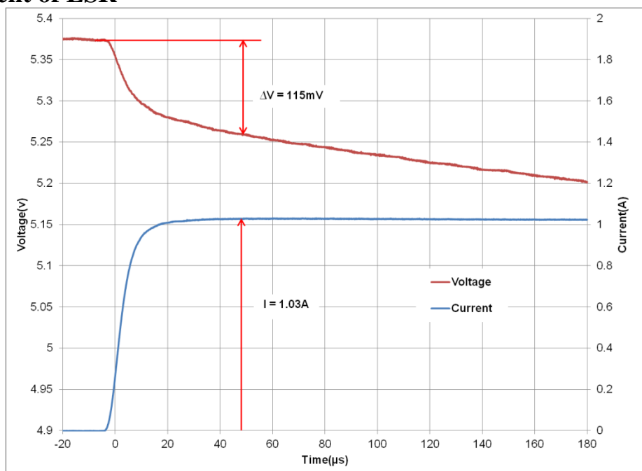
Fig 3: Measurement of ESR for an HA202
