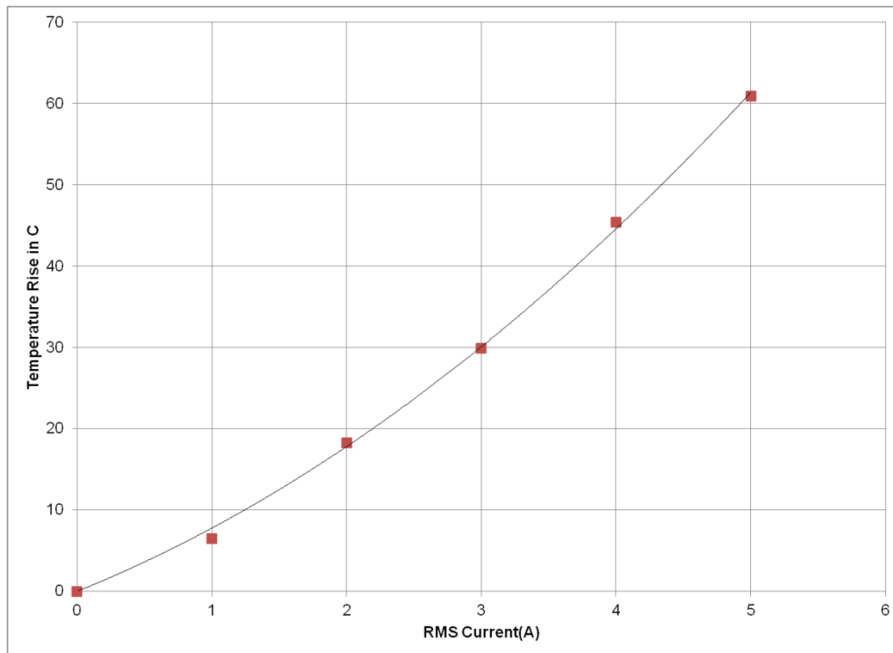
Fig 12: Temperature rise in HA202 with RMS current
