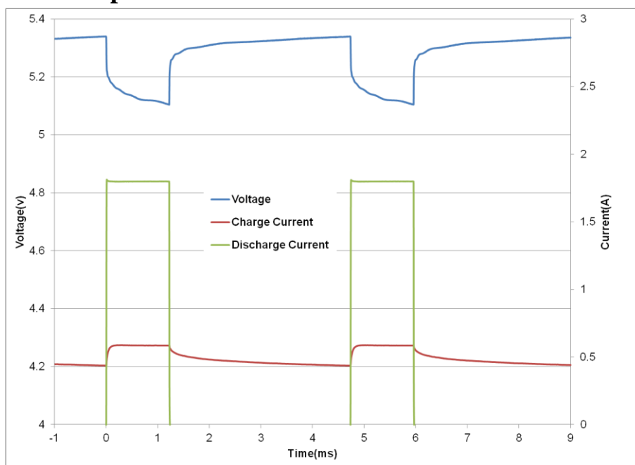
Fig 5: HA202 Pulse Response with GPRS Class 10 Pulse Train
